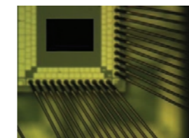
Brightfield Image
