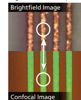
Brightfield Image
