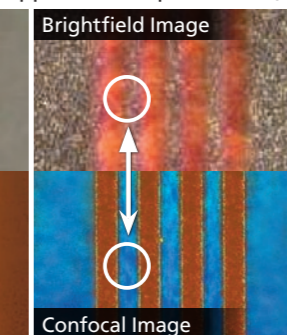
Confocal Image
